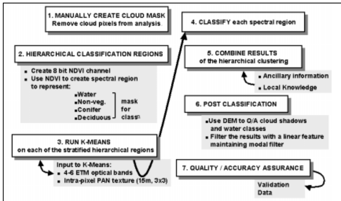
Fig. 1. Overview of EO SD Classification Methodology.
