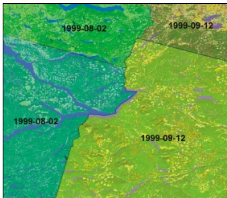
Fig. 4. Sample EOSD land cover product illustrating mosaic lines and source imagery (NTS 1:250 000 map sheet 93F (Nechako River, B.C.))
