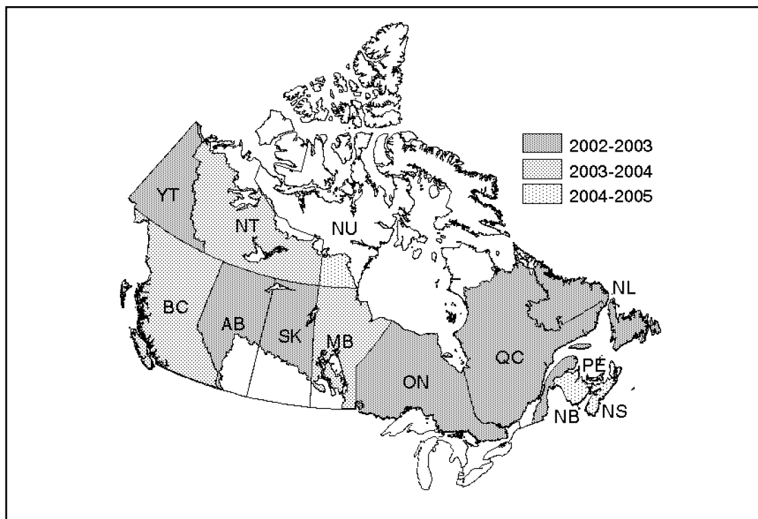
Fig. 2. Staged implementation, beginning in 2002, for the EOSD land cover mapping program.
