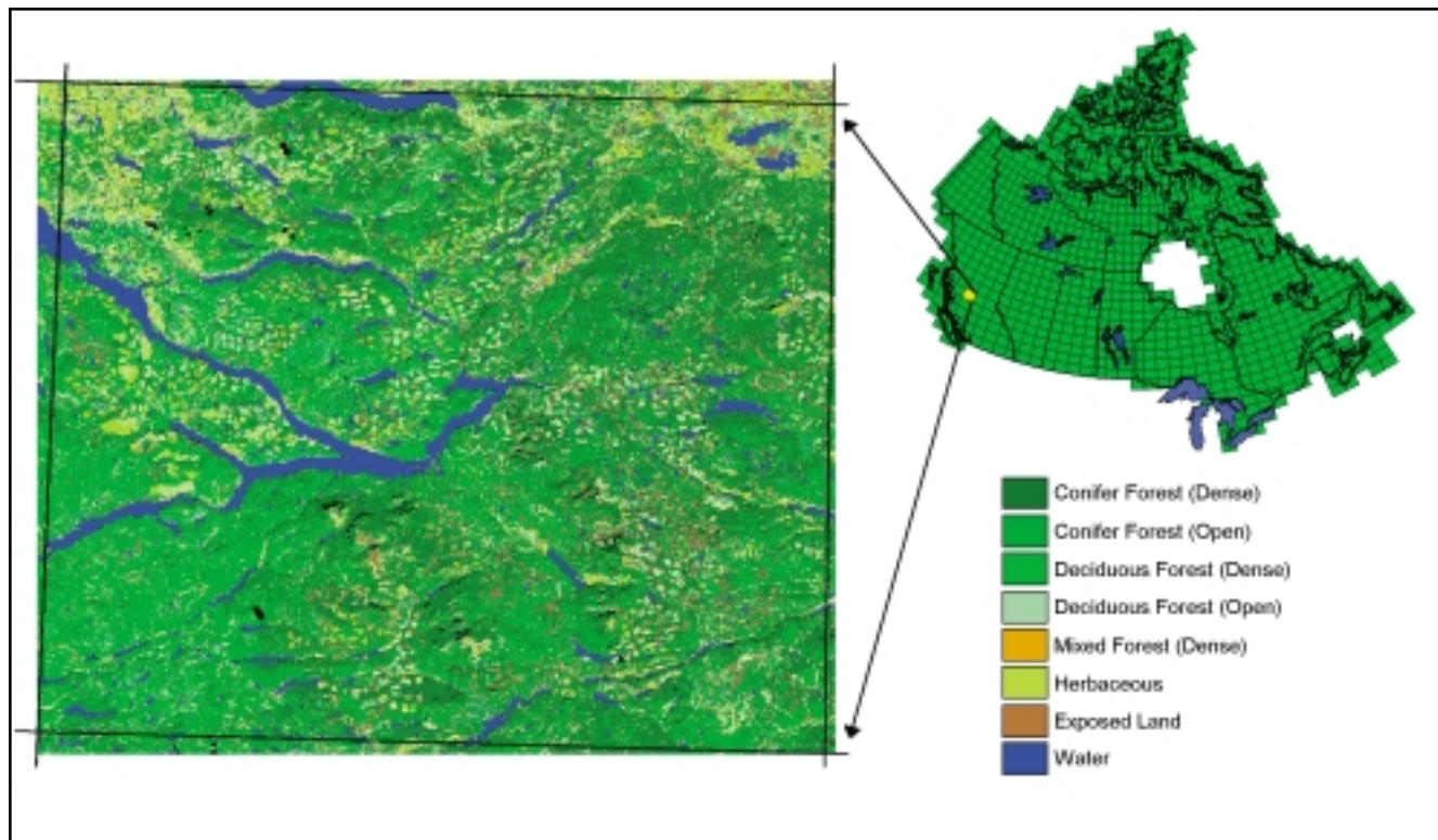
Fig. 3. Sample EOSD land cover classification product, representing same area as NTS 1:250 000 map sheet 93F (Nechako River, B.C.).
